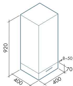
parete/wall
